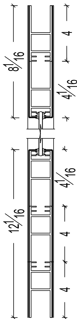
SIDE VIEW
