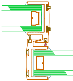
3 101.D HORIZONTAL CUT SECTION AT DOOR INTERLOCK STYLE REFERENCE
