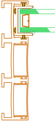
1 101.D HORIZONTAL CUT SECTION AT DOOR STRIKE REFERENCE
