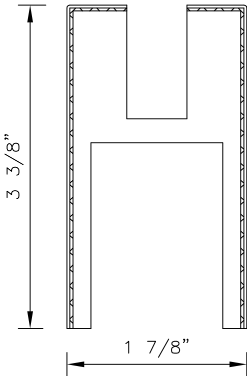
CLAD DETAIL
