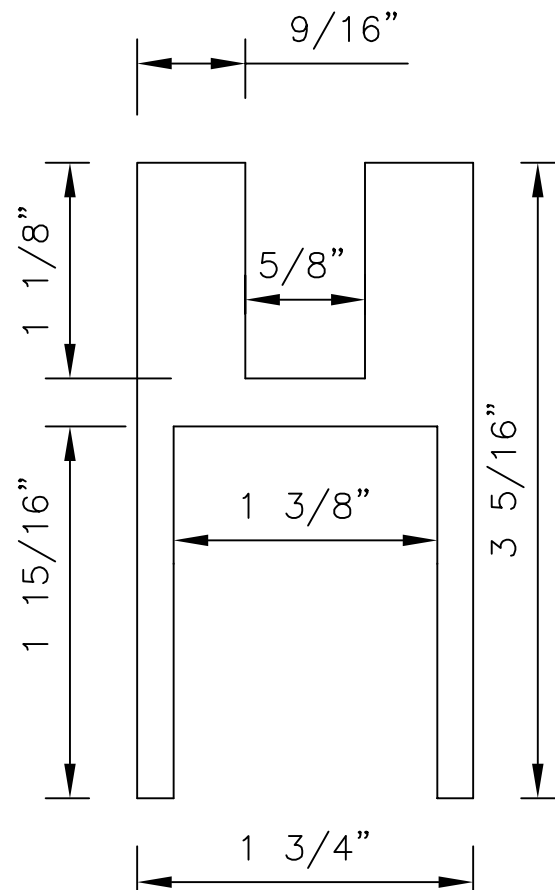
NON-CLAD DETAIL
