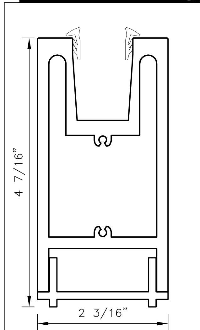
NON-CLAD DETAIL
