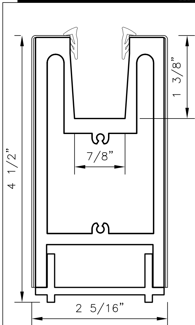
CLAD DETAIL
