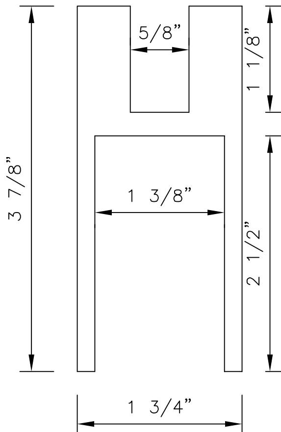
NON-CLAD DETAIL
