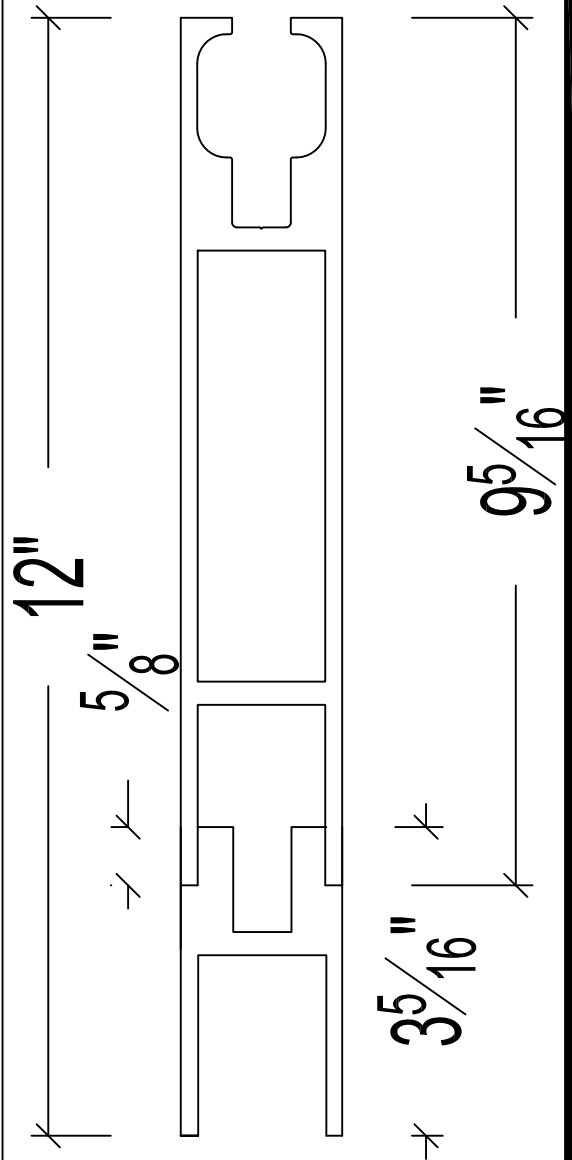
12" CUSTOM BTM RAIL
