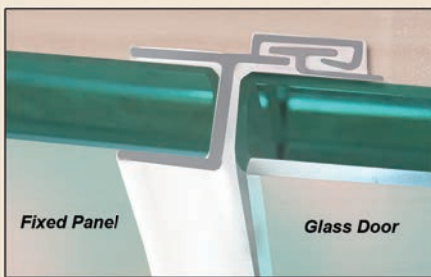
P180SDJ - 180 Deg. Strike Door 3/8" Glass
