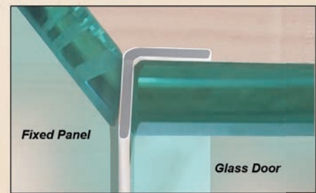
Multi-Purpose "H" Wipe 1/2" Glass
