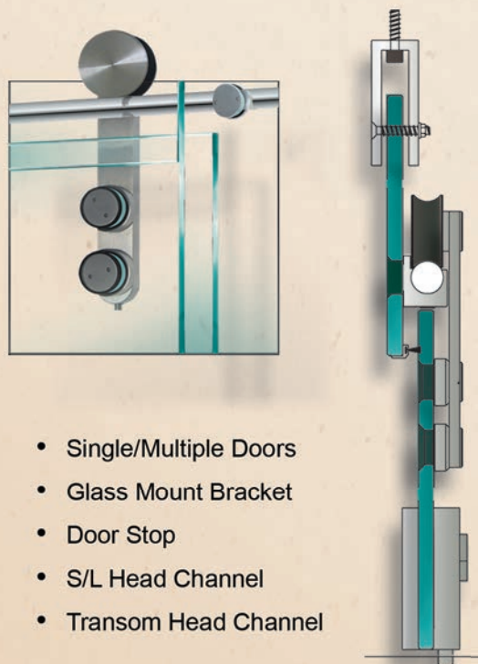
Ruby Glass Mount Slider with Easy Locking Ladder Pulls
